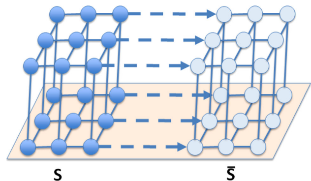
Fig. 1 A schematic illustration of a cut. The cut partitions the node set V into two disjoint sets: S and \bar{S} . The capacity C(S, \bar{S}) of the cut is the sum of the weights of the arcs that cross the cut, marked with a dashed line here
