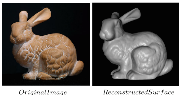
Fig. 6 Bunny problem instance—surface fitting (Source[49])
