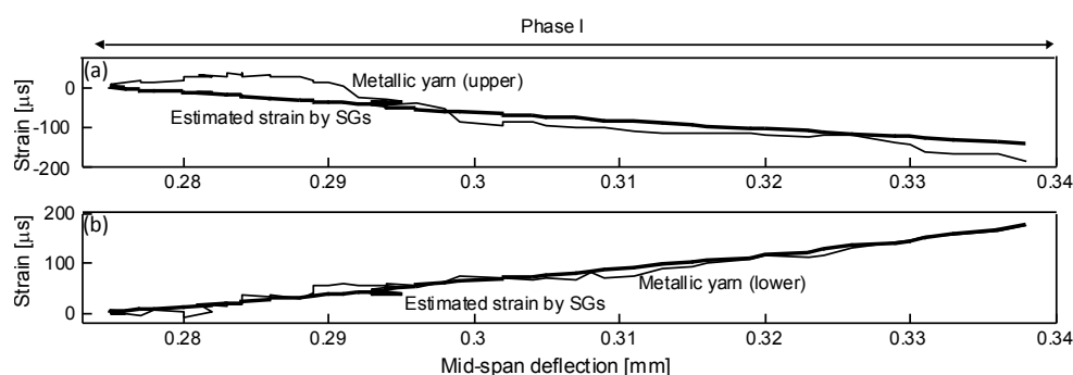
Figure 9: Strain reading of the metallic yarns in beam M1 compared with strains interpolated using the readings of the strain gauges (calibration factor= 25 \mu\epsilon/\mu V ): (a) upper yarns; (b) lower yarns.
