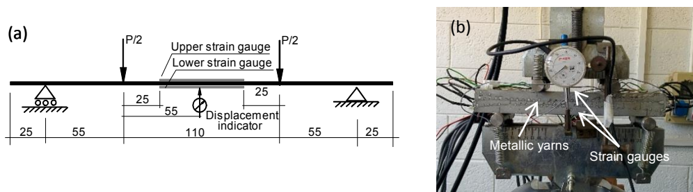
Figure 3: (a) Loading scheme and "external" sensing (adapted from [2]); (b) Test specimen and testing rig.
