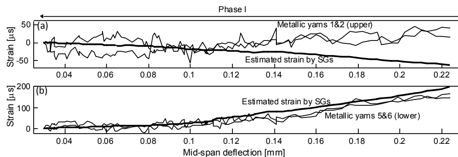
Figure 8: Strain reading of the metallic yarns in beam M2 compared with strains interpolated using the readings of the strain gauges (calibration factor= 45 \text{ } \mu\text{V}/\epsilon ): (a) upper yarns; (b) lower yarns.
